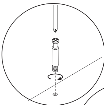
⑬ : Hanging Rail Support x 2
