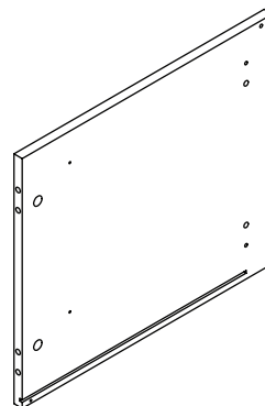
C : Right Side Panel x 1
