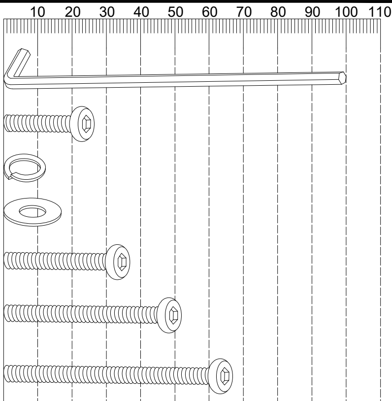
Fixtures and fittings supplied (actual size)
