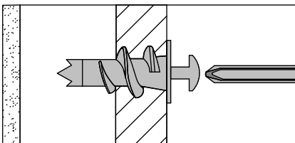
Nr.2 "Plasterboard" wall plug
