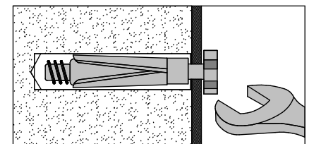
No.6 "Shield Anchor" wall plug Heavy load
