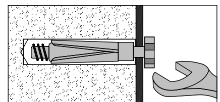
Taco de pared "Shield Anchor" No.6 Carga pesada
